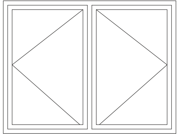
Double Butt Hinged Max Opening Angle: 170°±
